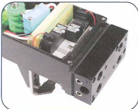
Solenoid valve and pneumatic manifold
